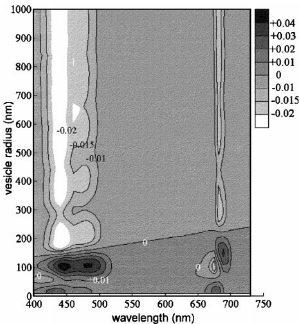
FIGURE 6 Contour plot of P^z(\lambda, r) , the fraction of light absorbed in the whole sphere, contributing to the z component of the sphere dipole moment, plotted as a function of wavelength \lambda and radius r . Positive values indicate an inverse light gradient, negative values a normal light gradient.
